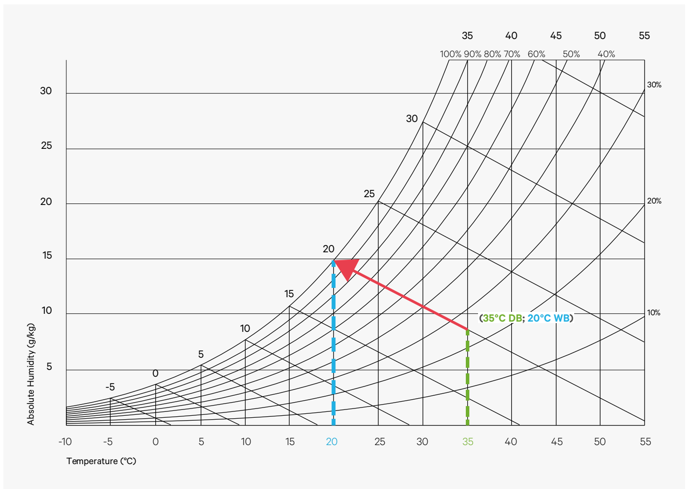
Figure 6. The Psychrometric Chart
